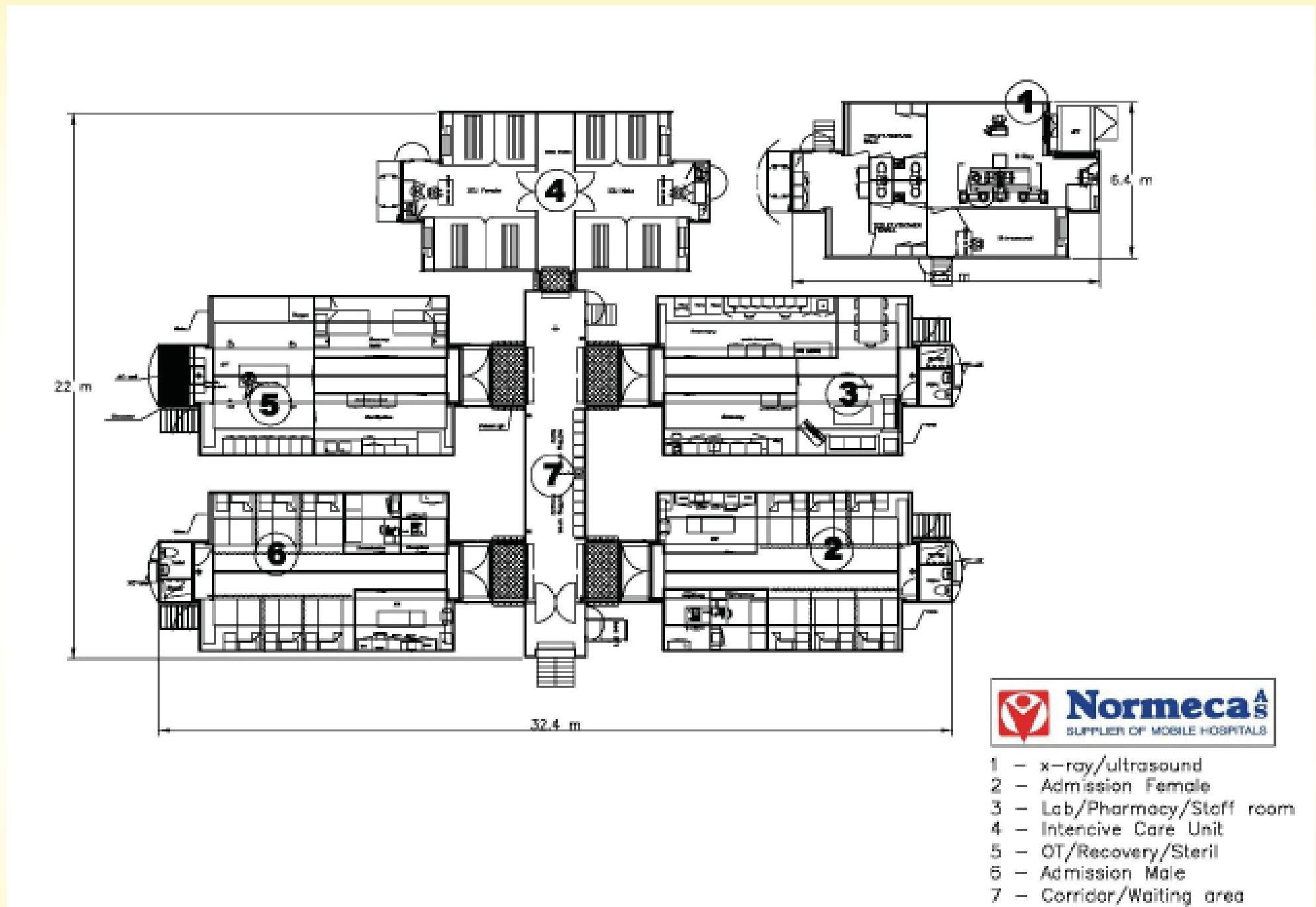
Drawing of the layout-plan for the hospital
