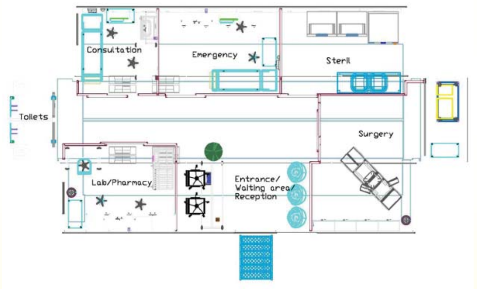
One trailer expandable on both sides.
